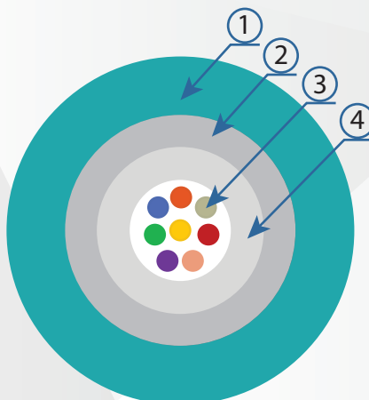
1 - LSOH jacket, 2 - Fiberglass, 3 - Optical fibers OM3, 4 - Tube with optical fibers
